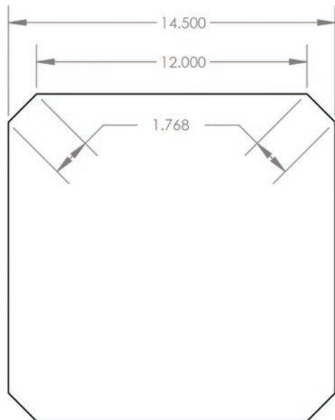
Island Top View SNK-15D / SSNK-15D
